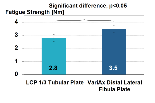
Fig. (11). Statistical evaluation of the fatigue testing showing significantly higher fatigue strength for the anatomically shaped plate.
