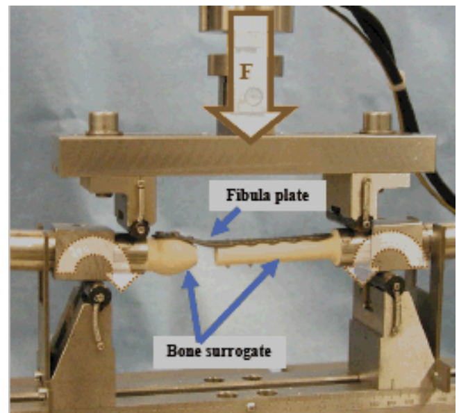
Fig. (4). Biomechanical test setup of the four point bending tests, F = applied cyclic load that results into a uniformly bending moment over the entire plate length.
