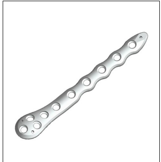
Fig. (8). Configuration of the designed implant in a computer sketch (five-hole version).
