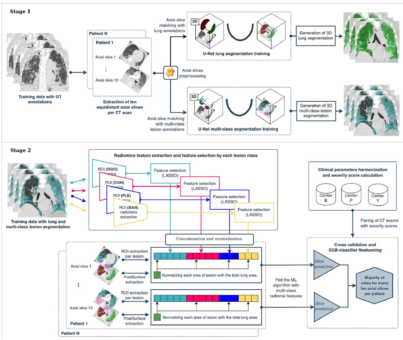
FIGURE 2. Overview of the AssessNet-19 model, a 2-stage pipeline for assessing COVID-19 patients' disease severity. First stage: Ten equidistant axial slices are extracted from each CT scan and paired with ground truth segmentation to train two 2D U-Net networks for lung and multiclass lesion segmentation. The 2D segmentation outputs are then used to construct the 3D volume of the lungs and multiclass lesions for quantification. Second stage: Radiomics feature extraction and selection process applied to each lesion class. Then, the elected features are concatenated, normalized, and inputted into the ML algorithm. Finally, the model was fine-tuned through cross-validation and XGB-classifier based on majority votes for every 10 axial slices per subject.
